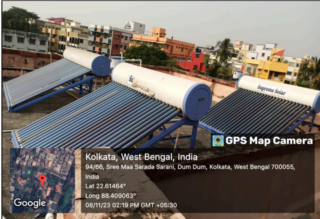
Supreme Solar Water Heater set up on 'Bharati Bhavan'
